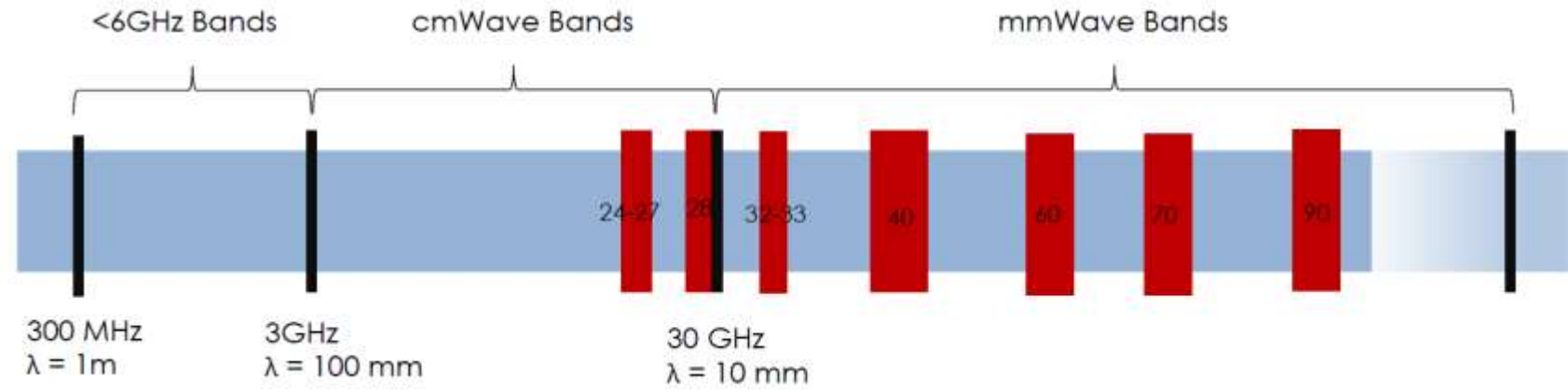
Spectrum band occupied by millimeter waves (Credit: Qualcomm )
